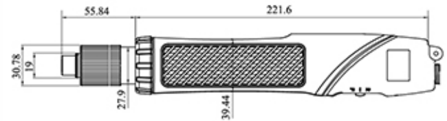
SKD-BN800P
